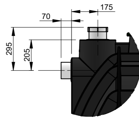
DETAIL A (INLET) SCALE 1 : 15
